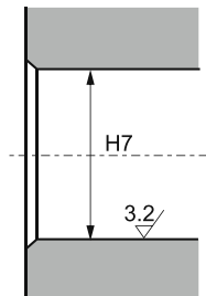
Mating Housing 相配座孔
